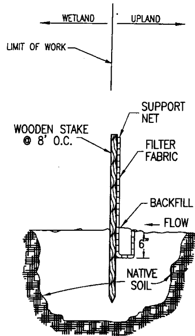
TYPICAL SILT FENCE DETAIL (NOT TO SCALE)
